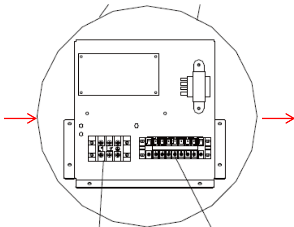
High voltage power supply Control wiring
